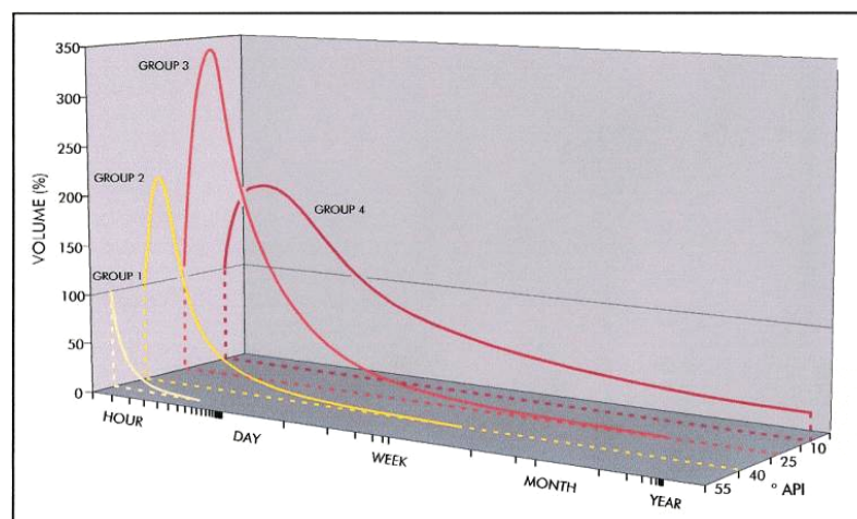
Figure 6.1: ITOPF model of oil types and behaviour
